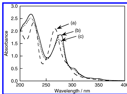
Figure 6. Absorption spectra of aqueous [Co(phen) 3 ]Cl 2 solutions (0.03 mmol L -1 ) (a) before photocatalytic reaction, (b) after H 2 evolution on Ru/SrTiO 3 :Rh photocatalyst, and (c) after overall water splitting by a (Ru/SrTiO 3 :Rh)–(BiVO 4 )–([Co(phen) 3 ] 3+/2+ ) system under visible light irradiation. Optical path length: 1 cm.
