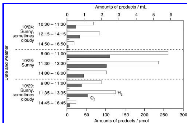
Figure 4. Solar water splitting by a (Ru/SrTiO 3 :Rh)–(BiVO 4 )–([Co(bpy) 3 ] 3+/2+ ) system. Reaction conditions: catalyst, 0.1 g each; starting reactant solution, 150 mL of an aqueous [Co(bpy) 3 ]SO 4 solution (0.2 mmol L -1 , initial pH: 3.8); light source, sunlight in autumn in Tokyo; irradiated area, 33 cm 2 . SrTiO 3 :Rh was prepared with Sr 3% excess and calcination at 1373 K.
