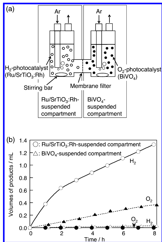
Figure 5. (a) Two-compartment-reactor for H 2 evolution separated from O 2 evolution. (b) H 2 evolution separated from O 2 evolution for overall water splitting by a (Ru/SrTiO 3 :Rh)–(BiVO 4 )–([Co(bpy) 3 ] 3+/2+ ) system. Catalyst: 0.1 g (Ru/SrTiO 3 :Rh), 0.3 g (BiVO 4 ), starting reactant solution: 0.5 mmol L -1 of an aqueous [Co(bpy) 3 ]SO 4 solution, 300 mL, initial pH adjusted to 3.8, light source: two 300 W Xe-arc lamps with cutoff filters (λ > 420 nm). SrTiO 3 :Rh powder was prepared by calcination at 1373 K with Sr 3% excess. Open and close marks indicate H 2 and O 2 , respectively.
