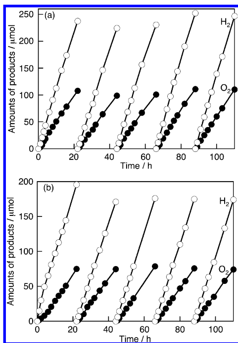
Figure 2. Overall water splitting under visible light irradiation by (Ru/SrTiO 3 :Rh)–(BiVO 4 ) systems employing (a) [Co(bpy) 3 ] 3+/2+ and (b) [Co(phen) 3 ] 3+/2+ electron mediators. Reaction conditions: catalyst, 0.1 g each; starting reactant solution, 120 mL of aqueous (a) [Co(bpy) 3 ]SO 4 and (b) [Co(phen) 3 ]Cl 2 solutions (0.5 mmol L -1 , initial pH: ~7); light source, a 300 W Xe-arc lamp with a cutoff filter ( \lambda > 420 nm); cell, top-irradiation type. SrTiO 3 :Rh was prepared by calcination at 1273 K without Sr excess.
