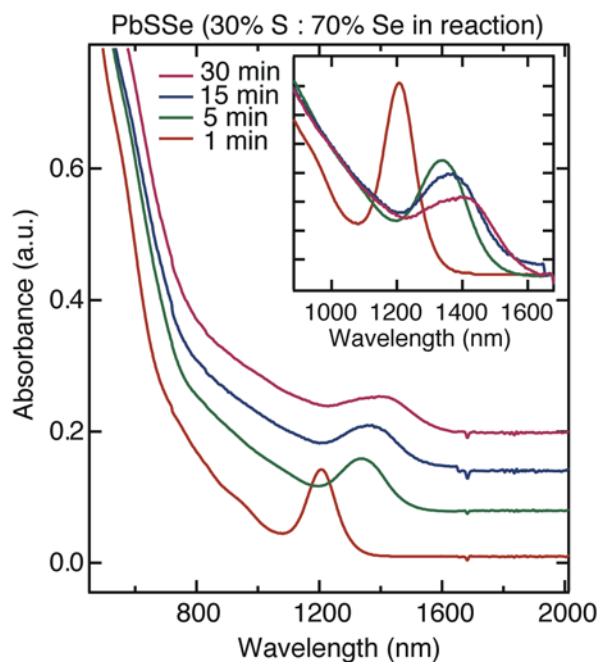
Figure S4. Absorbance of nanocrystals during the timed growth, offset for clarity. Subsequent growth times resulted in a broadened first exciton as well as a decrease in the bandgap. Since sharpest peaks are observed at short growth time, a reaction time of 90 seconds was used for all device work in the manuscript. Based on the width of the first exciton peak we estimate the dispersion in sample size to increase from below 10% to slightly greater than 20% after 30 mins.
