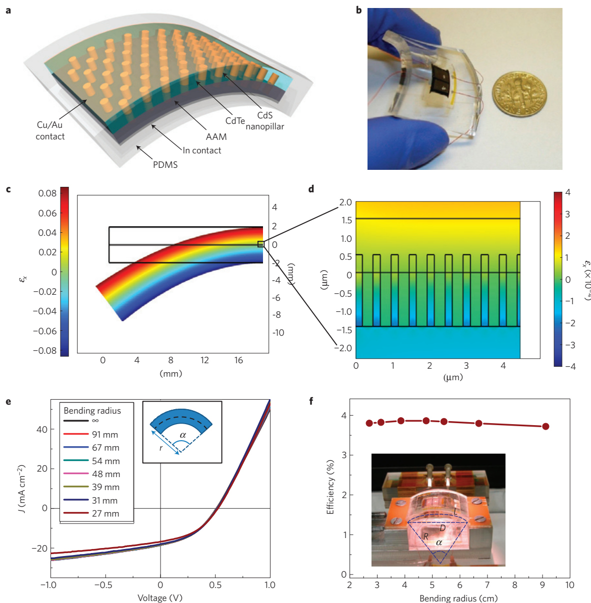
Figure 5 | Mechanically flexible SNOP cells. a, b Schematic diagram ( a ) and optical image ( b ) of a bendable SNOP module embedded in PDMS. c, d , Theoretical simulation of the strain for a flexible SNOP cell (PDMS thickness \sim 4 mm), showing only \sim 0.01\% maximum strain in the nanopillars. e , I - V characteristics of a flexible cell for various bending radii. f , Performance characterization of a flexible SNOP cell, showing minimal change in V_{oc} and \eta on bending of the substrate. The inset shows a picture of the set-up for bending the flexible modules.
