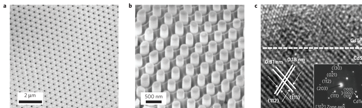
Figure 2 | SNOP cell at different stages of fabrication. a, b , SEM images of an as-made AAM with perfectly ordered pores ( a ) and a CdS nanopillar array after partial etching of the AAM ( b ). c , Transmission electron micrograph of the interface between a single-crystalline CdS nanopillar and a polycrystalline CdTe thin film. Inset: The corresponding diffraction pattern for which the periodically symmetric spots and multi-rings can be found. The symmetric spots are originated from the single-crystalline CdS nanopillar and the multi-rings are originated from the polycrystalline CdTe thin film.
