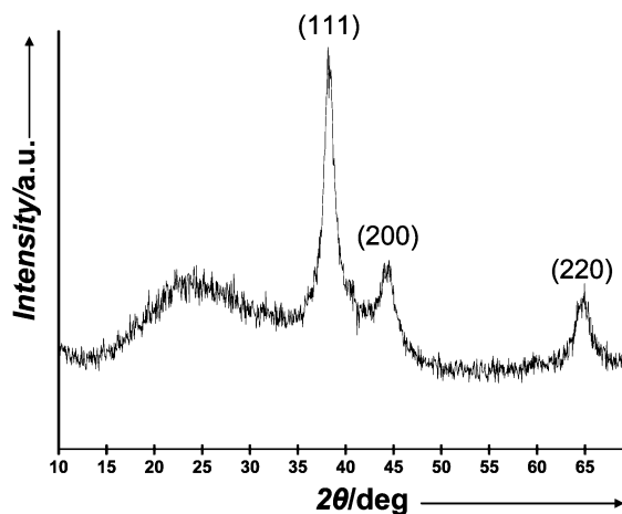
Figure 3. Powder X-ray patterns of the of the gold nanoparticles functionalized with boronic acid B-AuNPs. The broad peak at ca. 25^\circ is due to the scattering of the glass amorphous support.
