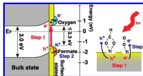
Figure 4. Schematic diagram showing electron transport triggered by light.
