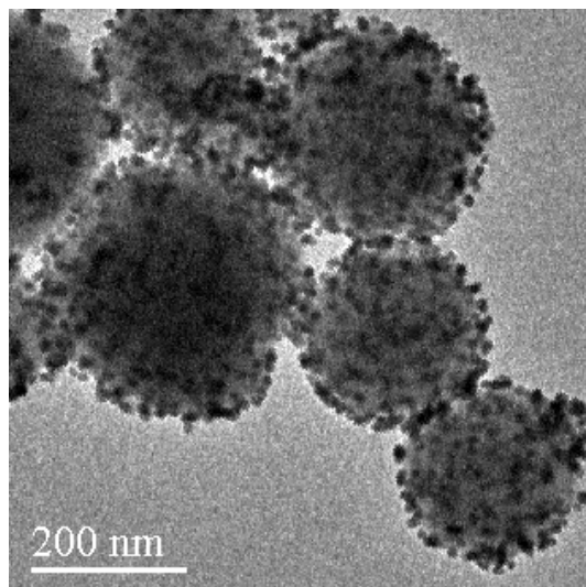
Figure S2. The TEM image of the Fe 3 O 4 @SiO 2 -Au microspheres with a low magnification, showing that the Fe 3 O 4 @SiO 2 microspheres were evenly decorated with Au nanoparticles of about 12 nm in size.
