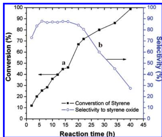
Figure 6. Epoxidation of styrene by using anhydrous t -butyl hydroperoxide (TBHP) as an oxidant over the \text{Fe}_3\text{O}_4@/\text{SiO}_2\text{-Au@mSiO}_2 microspheres with 90-nm thickness of mesoporous silica shells at 82 °C. The conversion of styrene and selectivity of styrene oxide were functioned with the reaction time.
