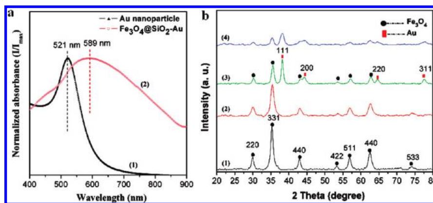
Figure 3. (a) UV-vis spectra of (1) Au nanoparticles aqueous dispersion (dark triangles) and (2) \text{Fe}_3\text{O}_4@/\text{SiO}_2\text{-NH}_2\text{-Au} microspheres aqueous dispersion (red cycles). (b) The wide-angle XRD patterns of (1) \text{Fe}_3\text{O}_4 particles, (2) \text{Fe}_3\text{O}_4@/\text{SiO}_2 microspheres, (3) \text{Fe}_3\text{O}_4@/\text{SiO}_2\text{-Au} microspheres, and (4) \text{Fe}_3\text{O}_4@/\text{SiO}_2\text{-Au@mSiO}_2 microspheres.
