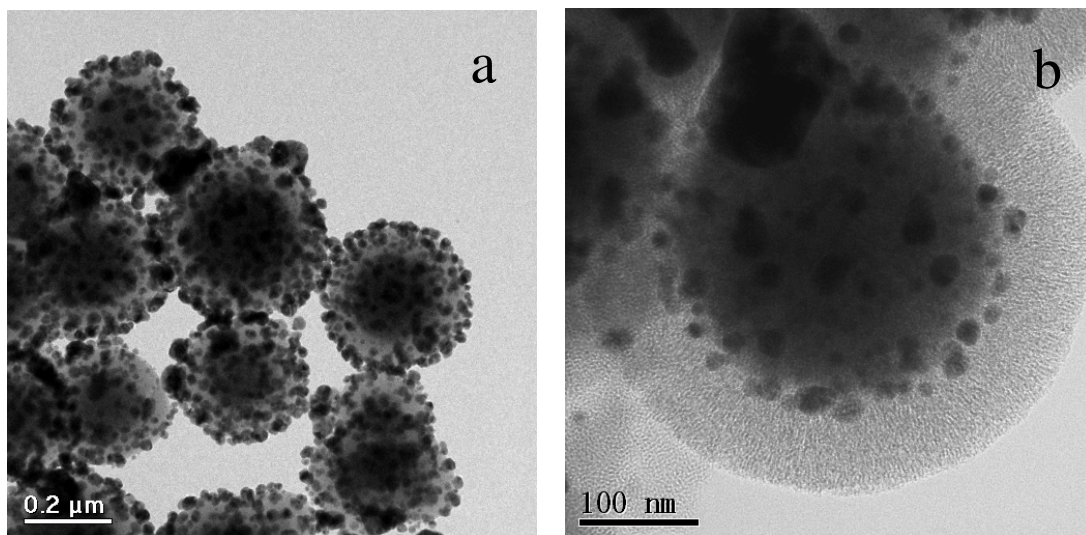
Figure S5. TEM images of (a) the \text{Fe}_3\text{O}_4@\text{SiO}_2\text{-Ag} particles and (b) \text{Fe}_3\text{O}_4@\text{SiO}_2\text{-Ag@mSiO}_2 microspheres.
