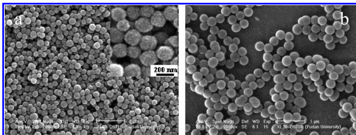
Figure 2. SEM images of the magnetite particles before (a) and after (b) the silica coating. Inset (a) is high-magnification SEM image.
