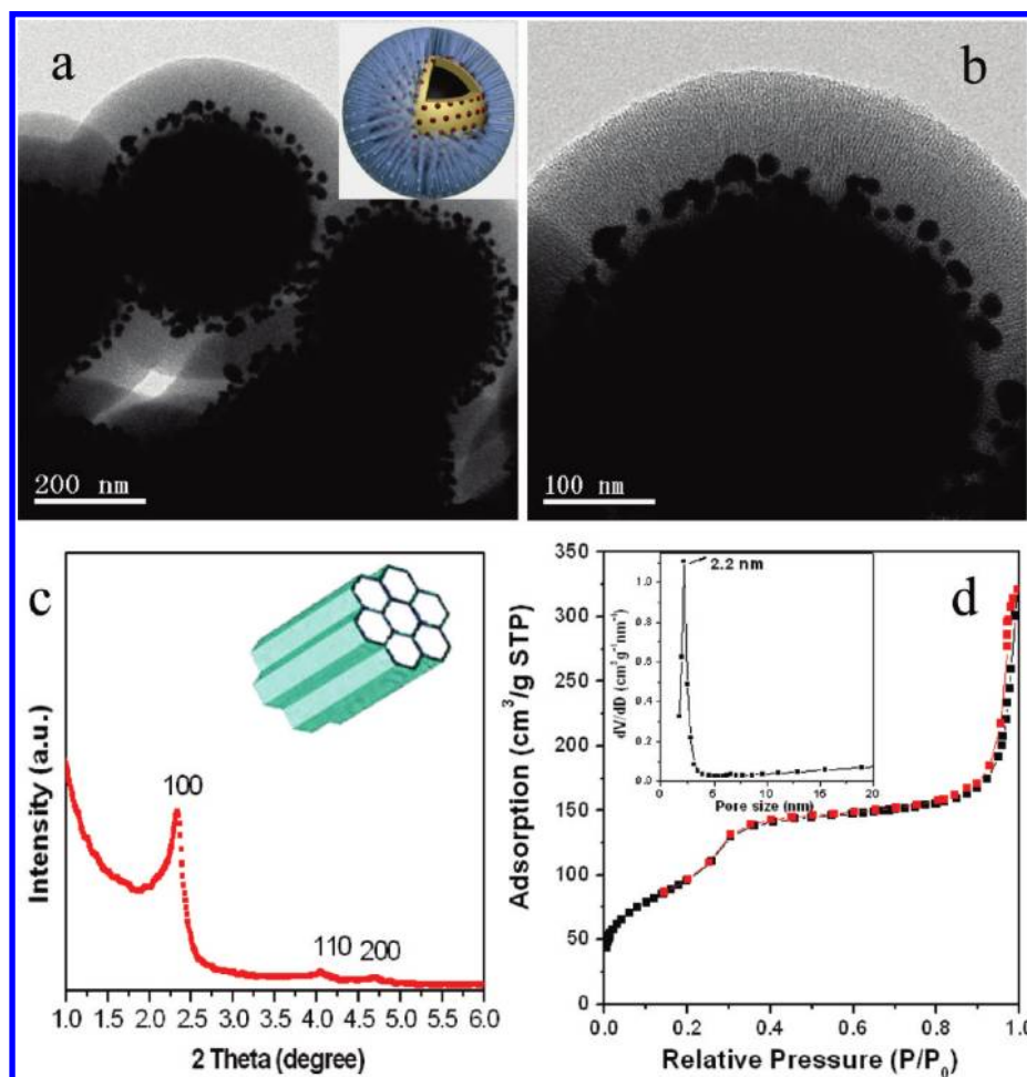
Figure 4. (a and b) TEM images of the Fe 3 O 4 @SiO 2 -Au@mSiO 2 microspheres with an 90-nm thick mesoporous silica layer, (c) the low-angle XRD pattern of the Fe 3 O 4 @SiO 2 -Au@mSiO 2 microspheres, (d) the nitrogen adsorption–desorption isotherms and pore size distribution (inset) of the Fe 3 O 4 @SiO 2 -Au@mSiO 2 microspheres with an 90-nm thick mesoporous silica layer. Inset (a) is a structural model of the Fe 3 O 4 @SiO 2 -Au@mSiO 2 microspheres; Inset (c) is a structural model of the mesoporous silica shells, showing 2-D hexagonal cylinder symmetry.
