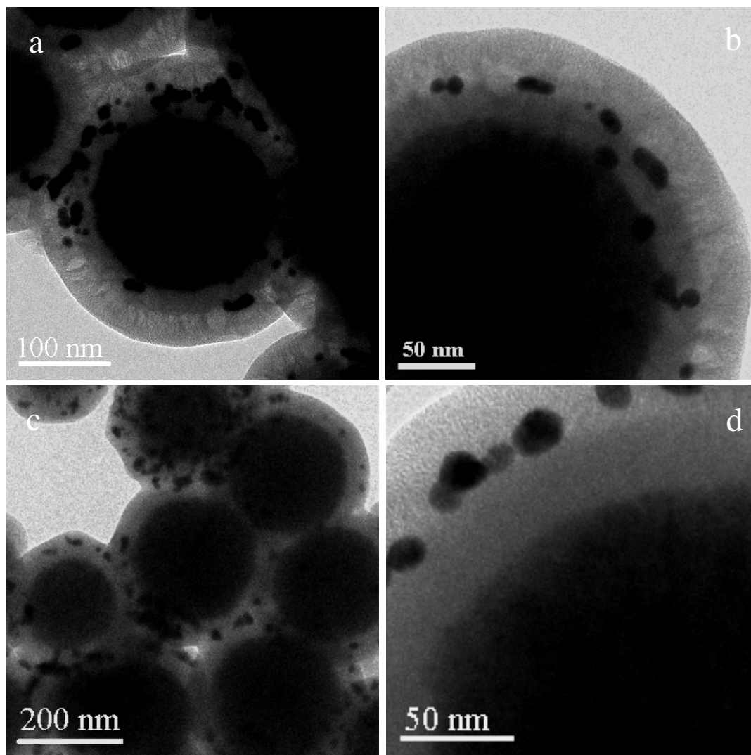
Figure S4. TEM images of the \text{Fe}_3\text{O}_4@ \text{SiO}_2\text{-Au@mSiO}_2 microspheres with (a, b) 40-nm and (c, d) 20-nm thick mesoporous silica shells, respectively.
