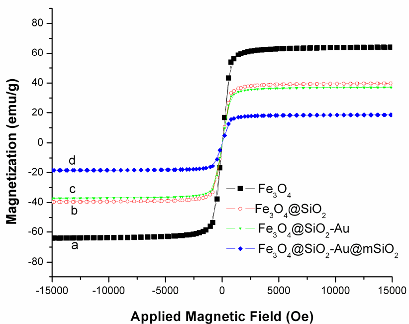
Figure S3. The magnetic hysteresis loops of (a) the \text{Fe}_3\text{O}_4 particles, (b) the core-shell \text{Fe}_3\text{O}_4@ \text{SiO}_2 microspheres, (c) the \text{Fe}_3\text{O}_4@ \text{SiO}_2\text{-Au} microspheres and (d) the \text{Fe}_3\text{O}_4@ \text{SiO}_2\text{-Au@mSiO}_2 microspheres with 90-nm thickness outer mesoporous silica layer.
