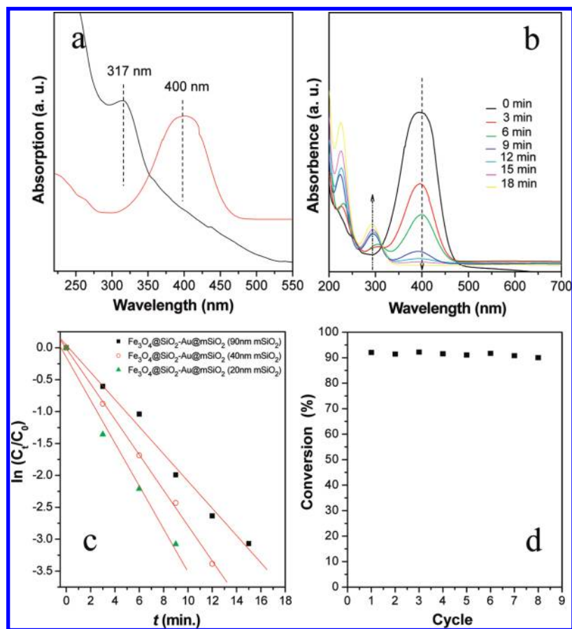
Figure 5. (a and b) UV-vis spectra of (a) 4-nitrophenol before and after adding NaBH 4 solution, (b) the reduction of 4-nitrophenol in aqueous solution recorded every 3 min using the Fe 3 O 4 @SiO 2 -Au@mSiO 2 microspheres (90-nm thick mesoporous silica shell) as a catalyst, (c) the relationship between ln(C t /C 0 ) and reaction time ( t ), wherein, the ratios of 4-NP concentrations (C t at time t ) to its initial value C 0 ( t = 0) were directly given by the relative intensity of the respective absorbance A t /A 0 , and therefore, the reduction course could be directly reflected by these absorption curves. (d) The reusability of the Fe 3 O 4 @SiO 2 -Au@mSiO 2 microspheres (90-nm thickness of mesoporous silica shells) as a catalyst for the reduction of 4-nitrophenol with NaBH 4 .
